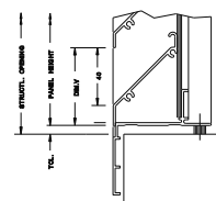
551. VARI-BLADE CILL DETAIL
