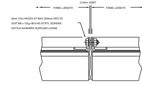
553. HORIZONTAL JOINT DETAIL
