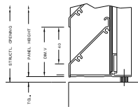
559. VARI-BLADE CILL DETAIL
