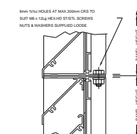
55X. VERTICAL JOINT DETAIL
