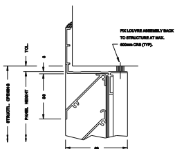
550. STANDARD HEAD DETAIL
