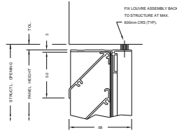
558. STANDARD HEAD DETAIL
